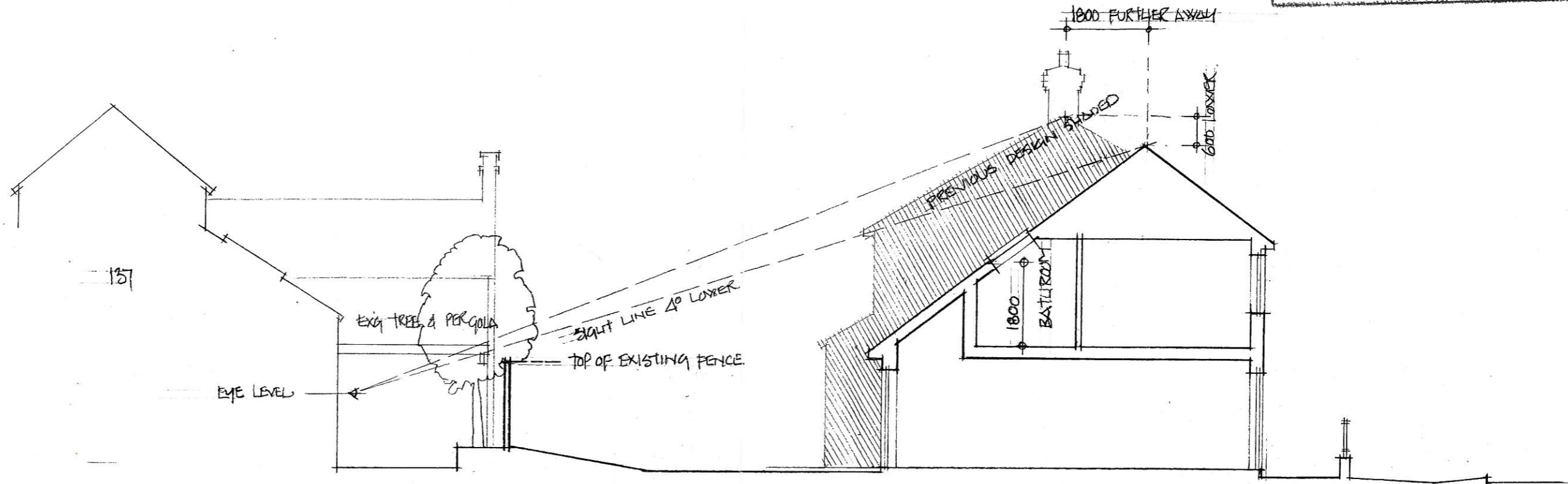
5 BELLS SITE RECONFIGURED : SKETCH SECTION THRU PLOT 1. : 1:100 SK 110720 A
